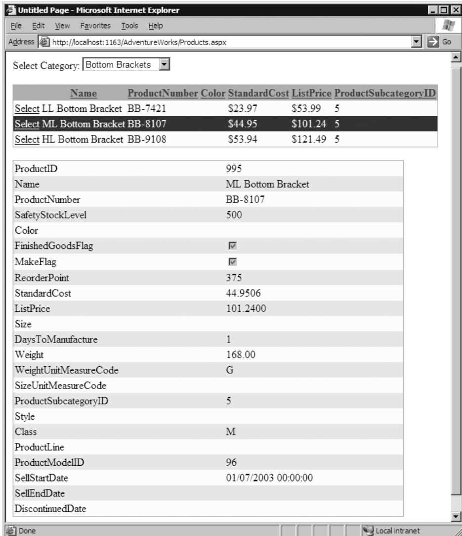
FIGURE 2.22: The results from using a data access/business logic layer
