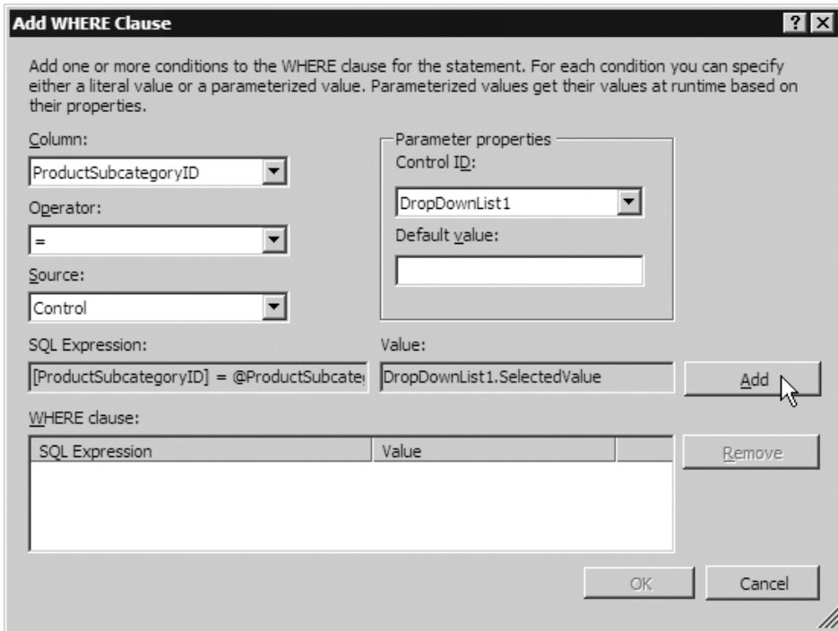
FIGURE 2.12: Adding a WHERE clause to select on subcategory
