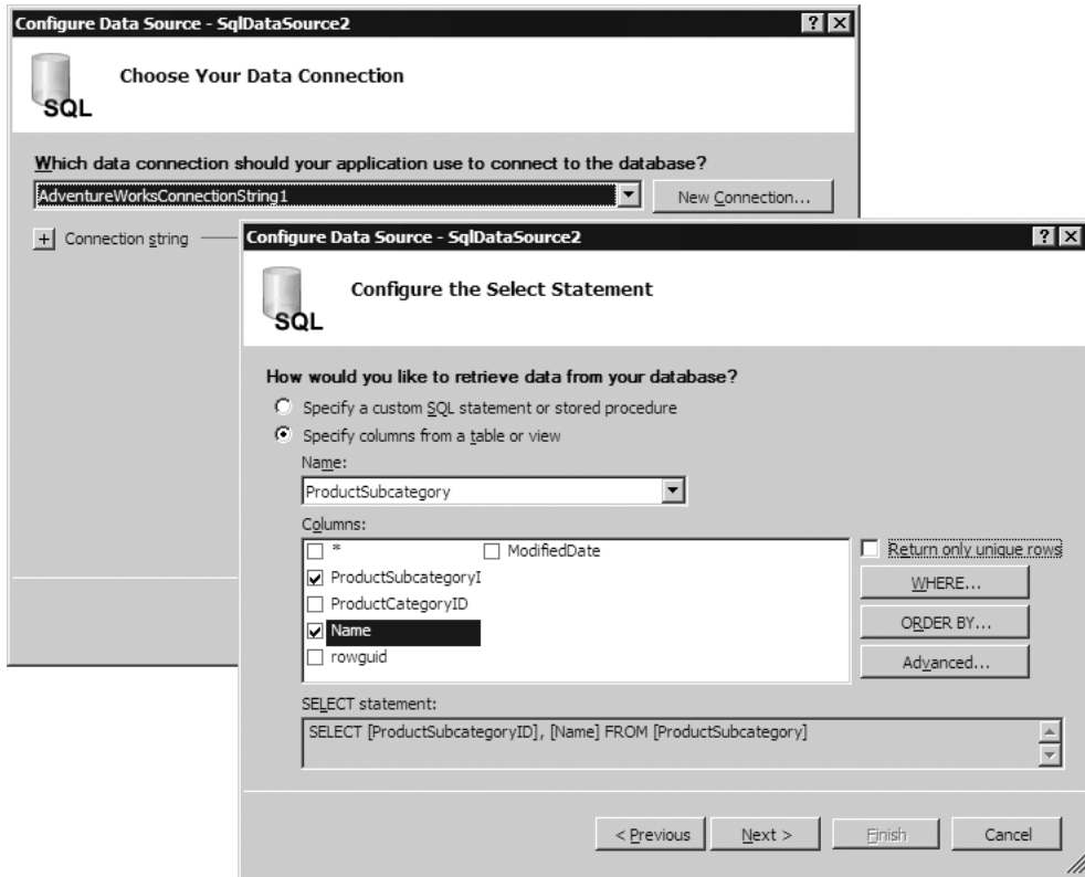
FIGURE 2.10: Setting the properties of the new SqlDataSource to select the category details
