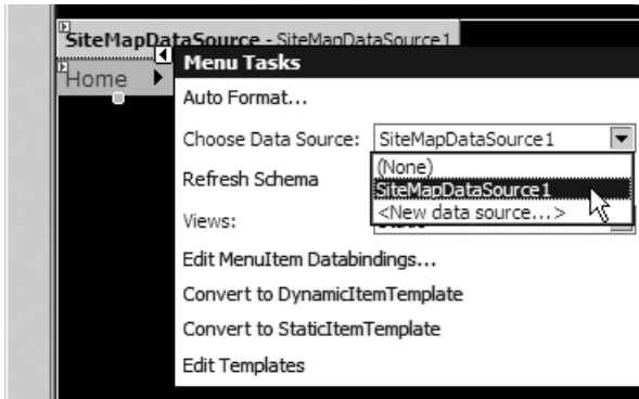
FIGURE 2.25: Adding a SiteMapDataSource and menu control to the Master Page
