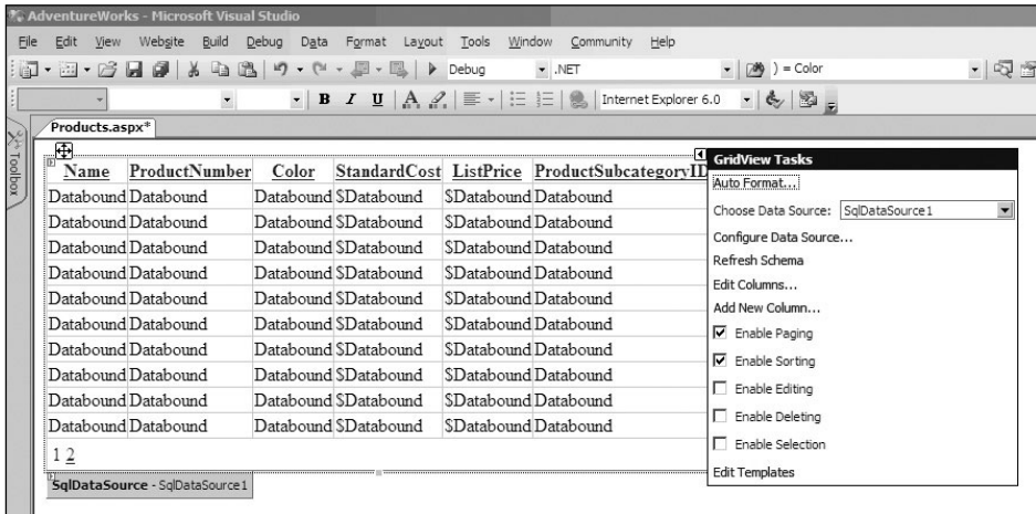
FIGURE 2.6: Enabling sorting and paging in the GridView tasks pane
