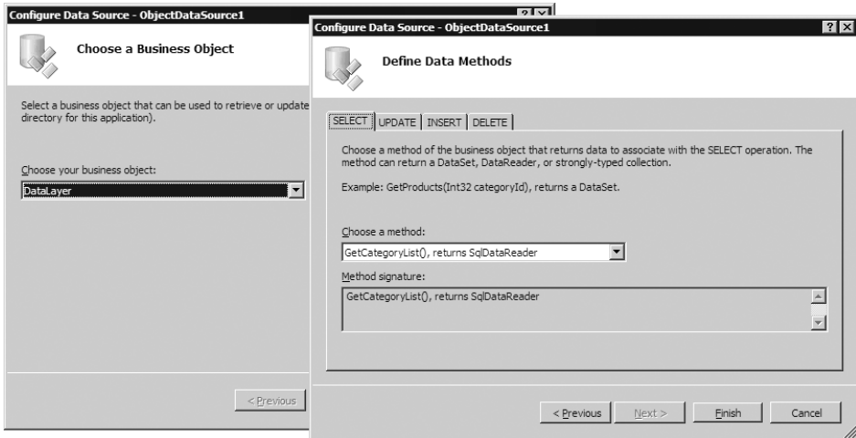
FIGURE 2.19: Configuring the ObjectDataSource for the DropDownList
