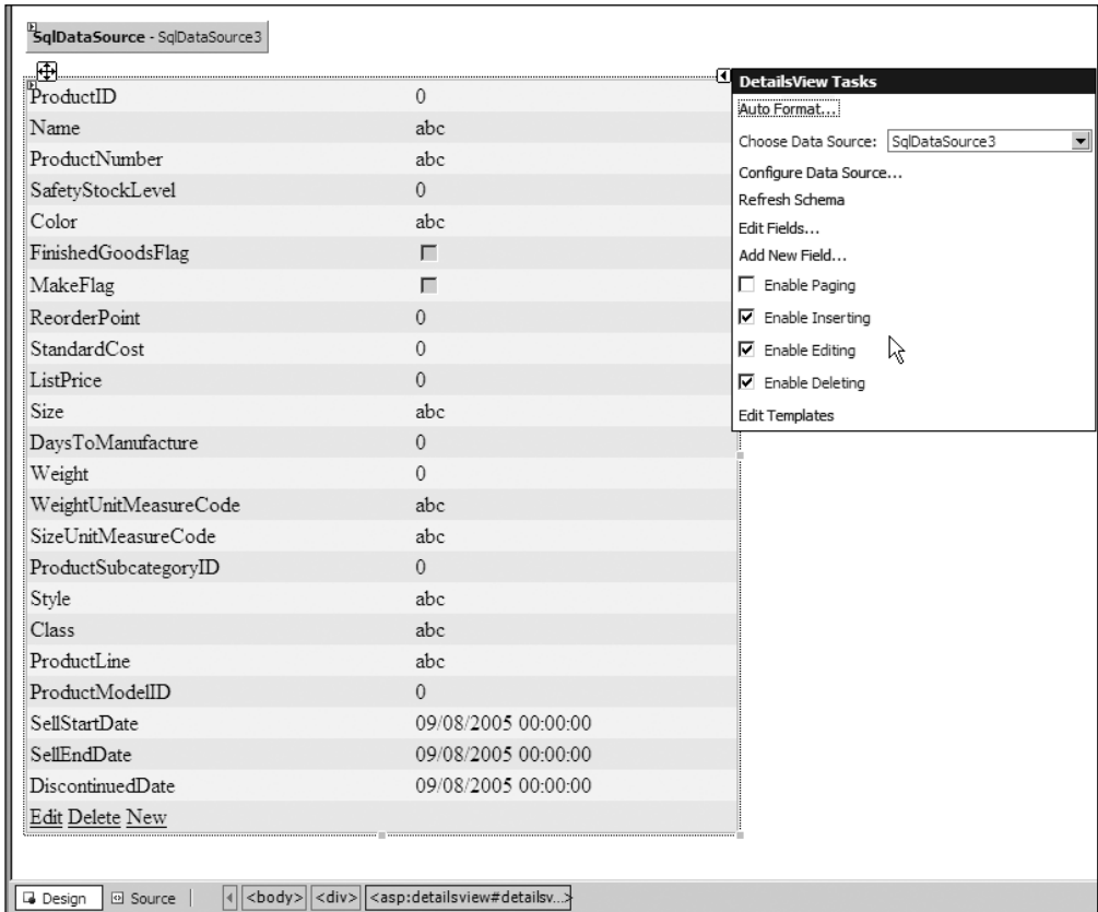
FIGURE 2.17: Setting the editing options for the DetailsView control
