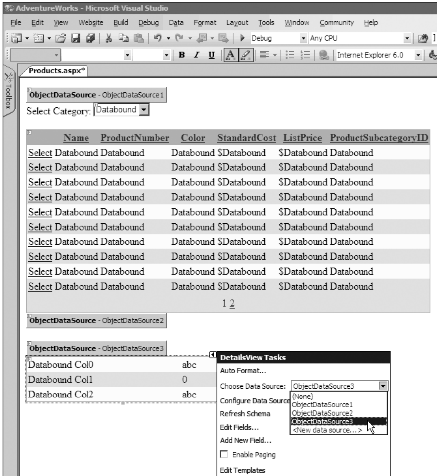
FIGURE 2.21: Connecting the data display controls to the ObjectDataSource instances
