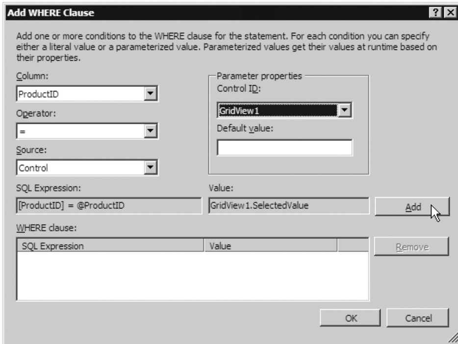
FIGURE 2.15: Creating a ControlParameter for the third SqlDataSource control
