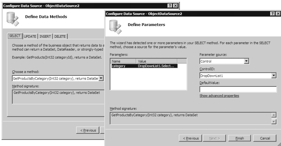
FIGURE 2.20: Configuring the ObjectDataSource for the GridView
