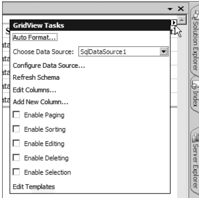
FIGURE 2.4: Opening the Tasks pane in Visual Studio and Visual Web Developer
