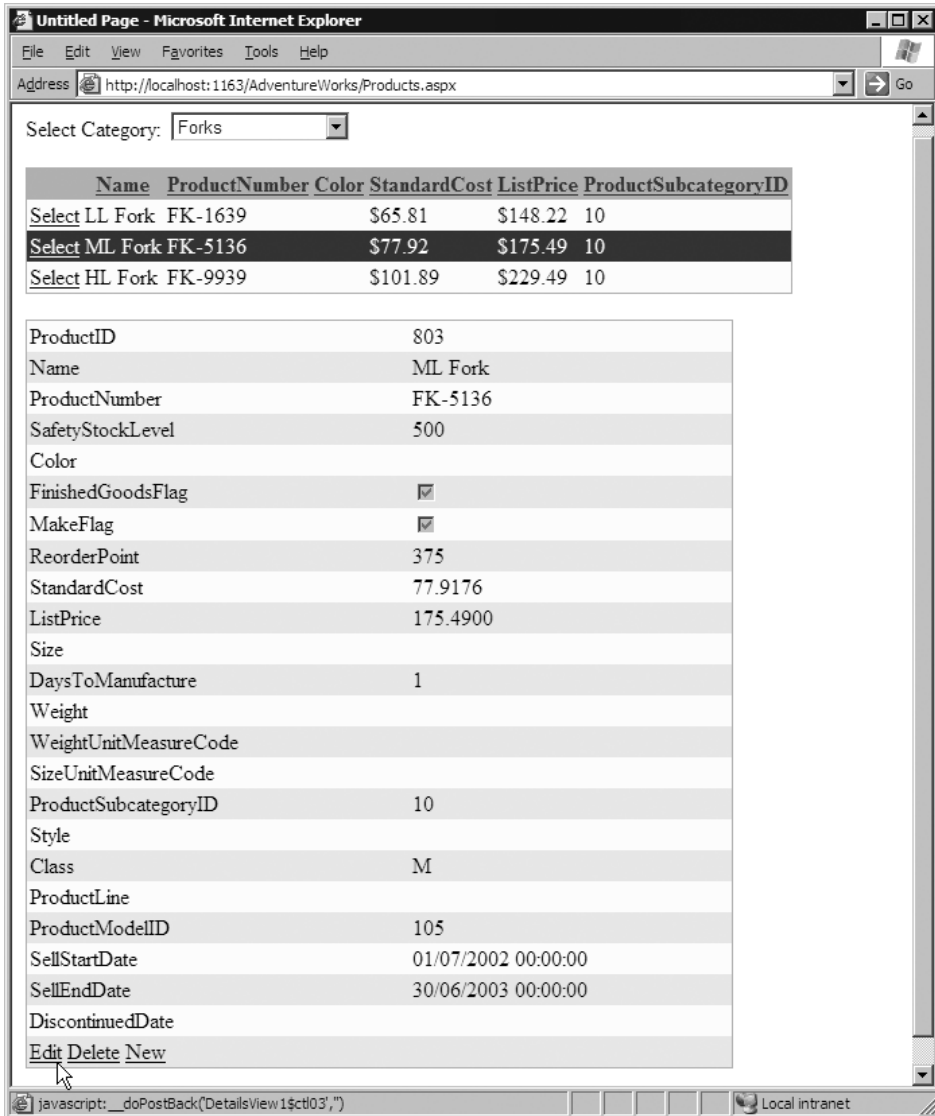
FIGURE 2.18: Viewing and editing rows in a linked DetailsView control
