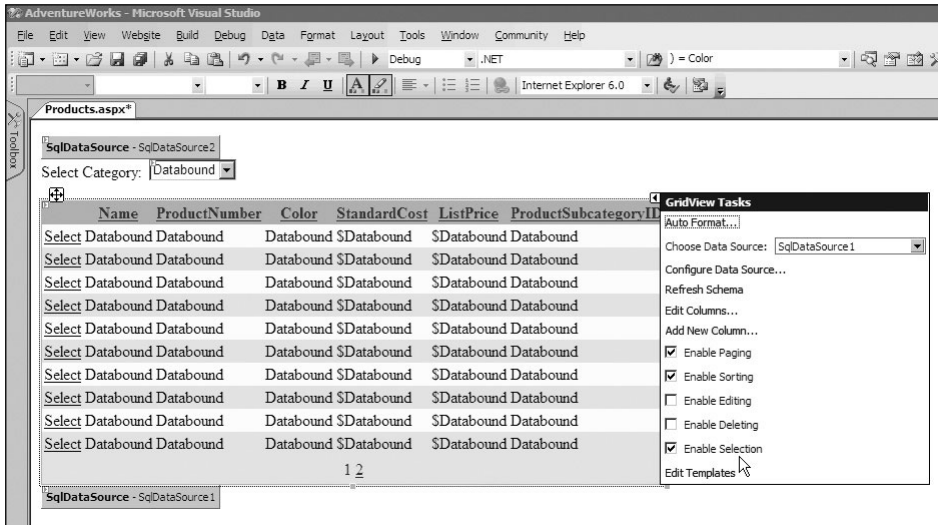
FIGURE 2.14: Specifying selection without editing features for a GridView control
