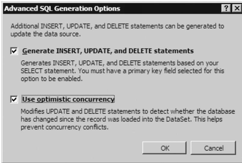
FIGURE 2.16: Specifying the options to allow row updates through controls linked to this SqlDataSource
