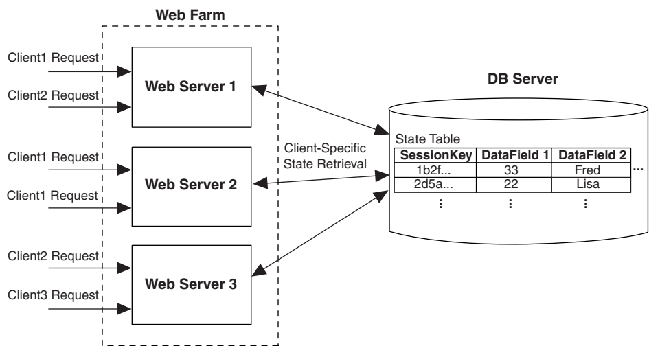
FIGURE 10-3: Maintaining Client-Specific State in a Web Farm Deployment
