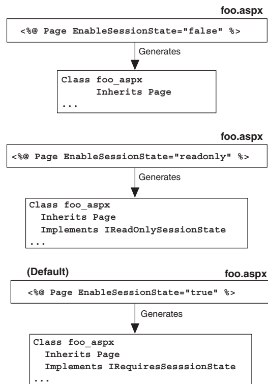
FIGURE 10-6: Indicating Session State Serialization Requirements in Pages
